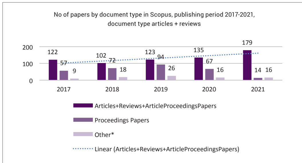
Figure 5. WOS– Total number of papers by publishing year and document type
