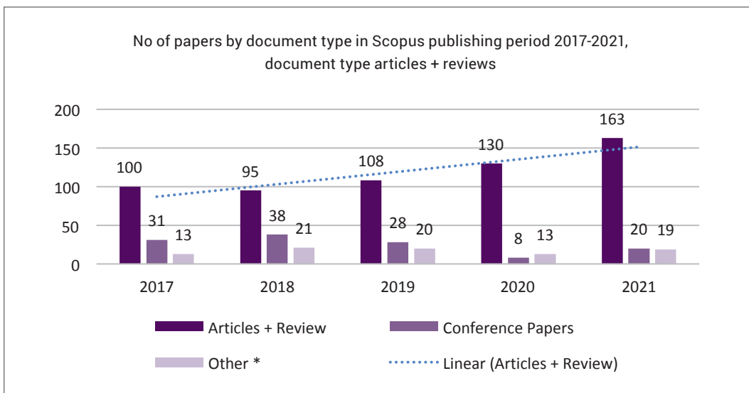
Figure 3. Scopus – Total number of papers by publishing year and document type
