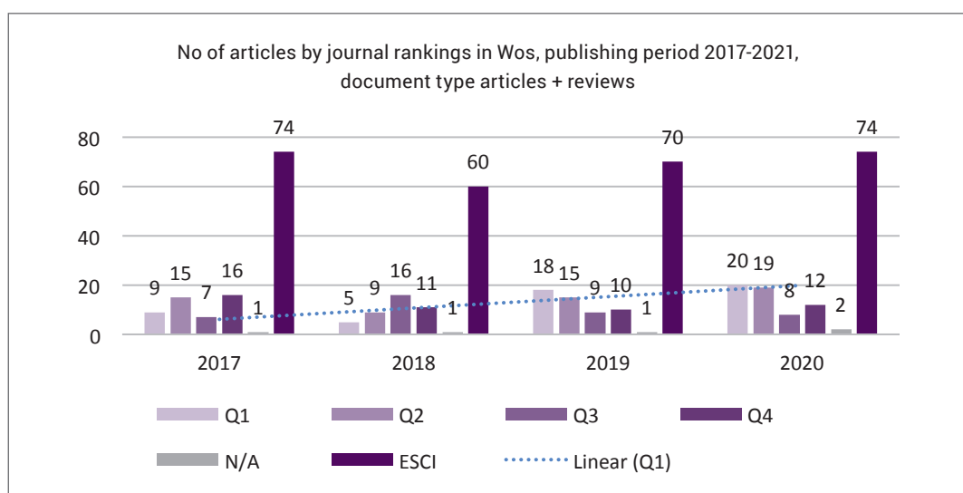
Figure 4. WoS -Total number of WoS articles by publishing year and quartiles
