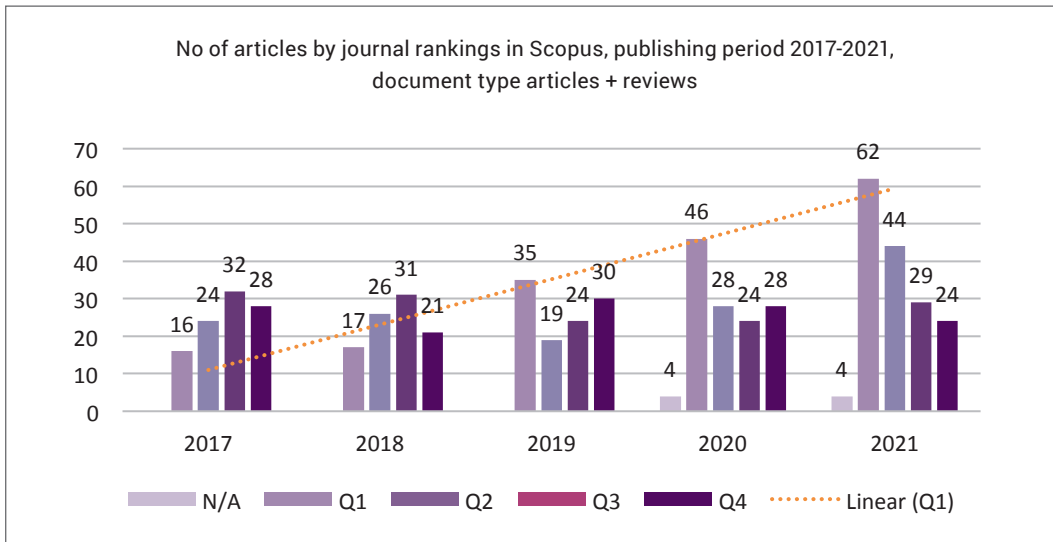
Figure 2. Scopus - Total number of Scopus articles by publishing year and quartiles
