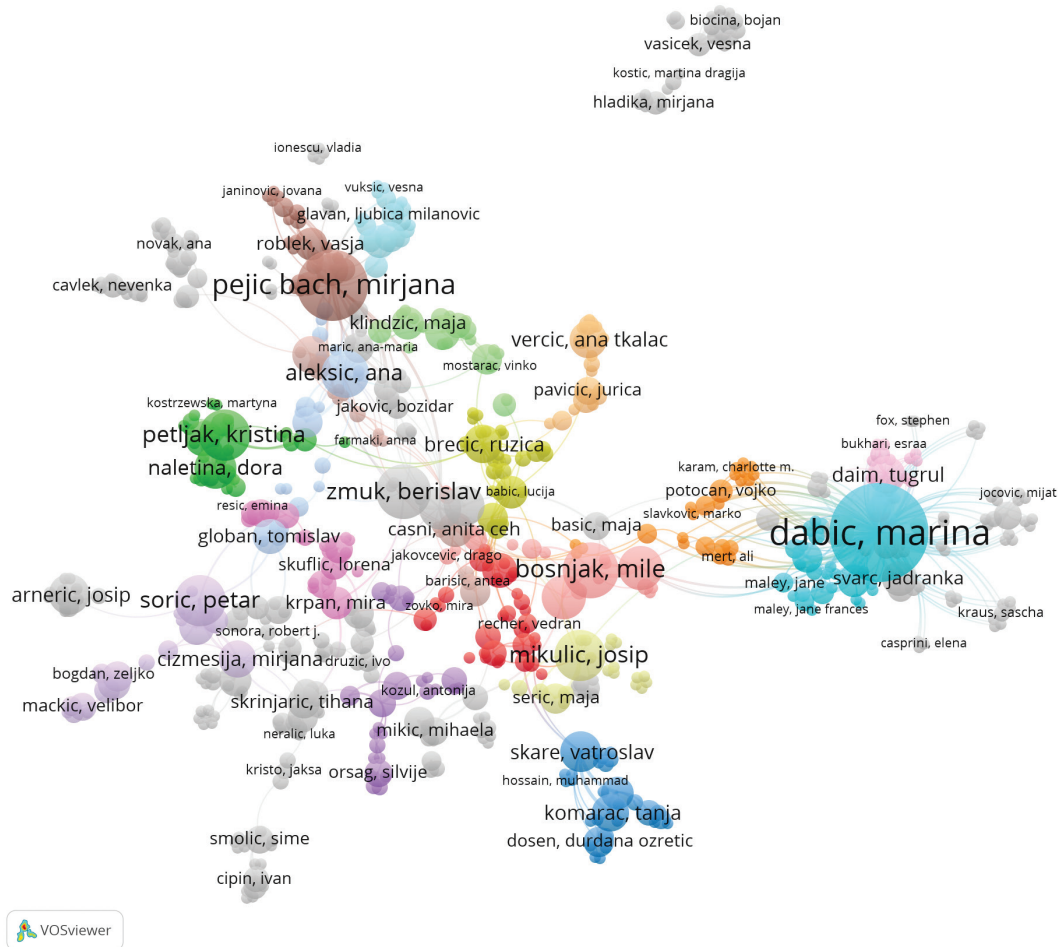
Figure 7. FEB's authors referenced in WOS and their strongest cooperation
