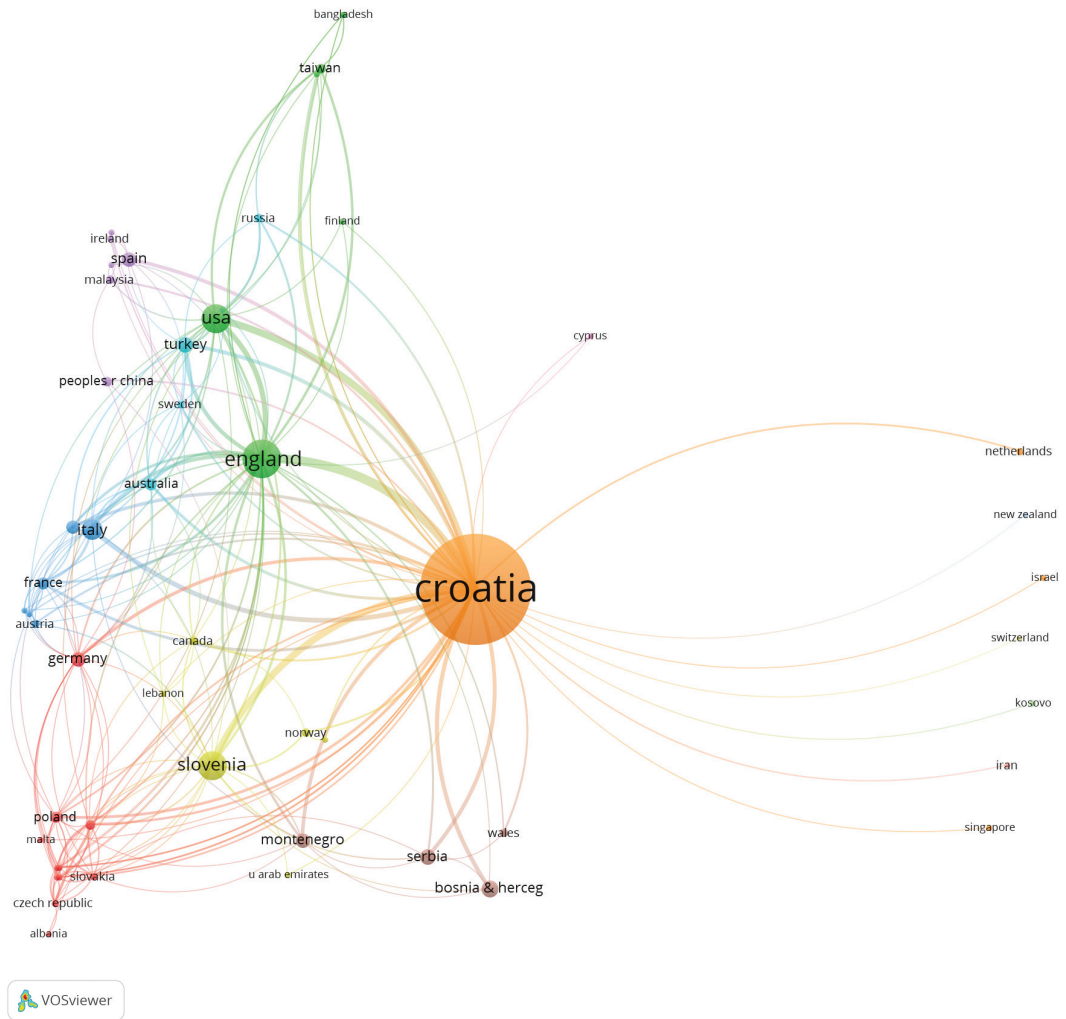
Figure 8. Embedding engagement in international research
